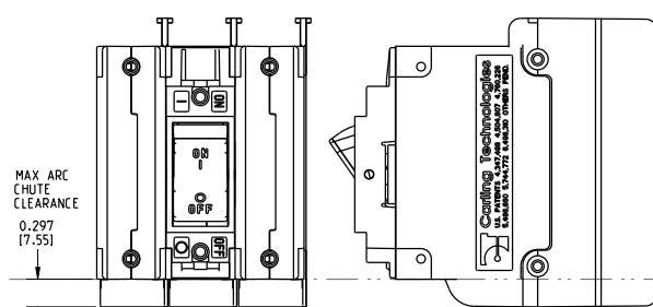
3-POLE (CF3,CG3,C13,C23) w/ ARC CHUTE BARRIER
