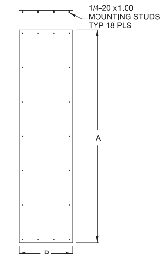
Flat End Plate
