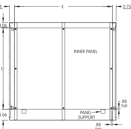
Rear View (Cross Section)
