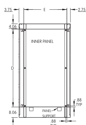
Rear View (Cross Section)
