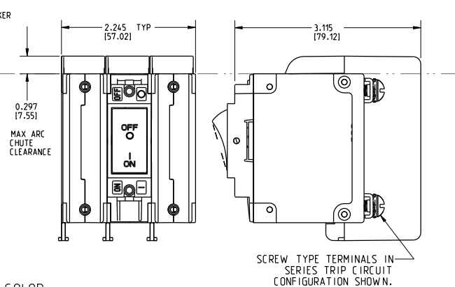
3-POLE (CF3,CG3,C13,C23) w/ ARC CHUTE BARRIER
