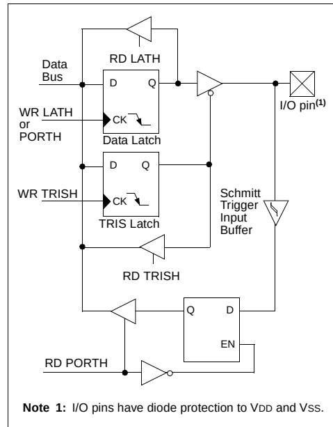
FIGURE 9-16: RH3:RH0 PINS BLOCK DIAGRAM IN I/O MODE
