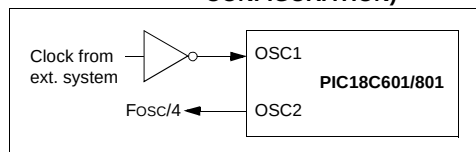
FIGURE 2-3: EXTERNAL CLOCK INPUT OPERATION (EC OSC CONFIGURATION)
