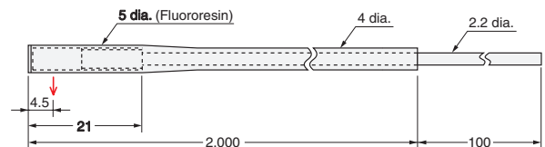
E32-T81F-S (R10)
