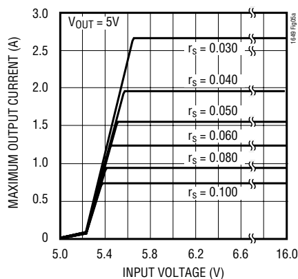
Figure 5a. MAX1649 Current-Sense Resistor Graph
