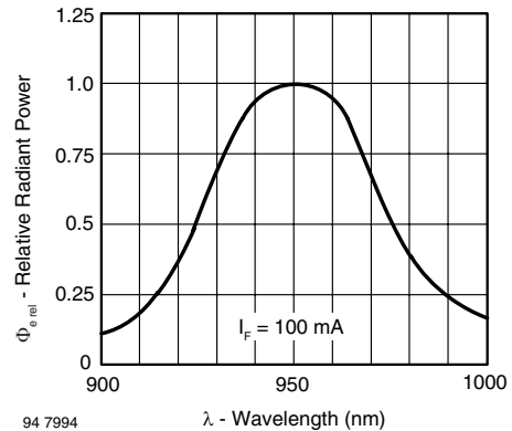
94 7994 \lambda - Wavelength (nm) Fig. 9 - Relative Radiant Power vs. Wavelength
