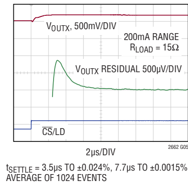
Settling 145mA to 155mA Step
