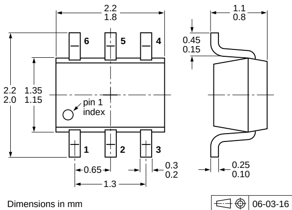
Fig 11. Package outline PUMH18 (SOT363)
