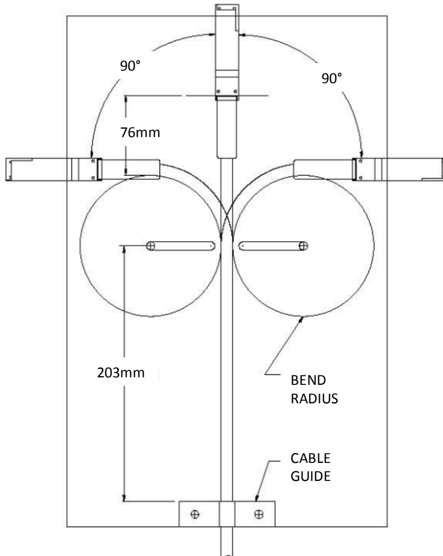
Figure 3 – Repeated Wire Flex Test (See Mechanical Characteristics 8.7 and Table 1)
