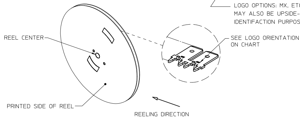
DETAIL 1 SCALE 20:1
