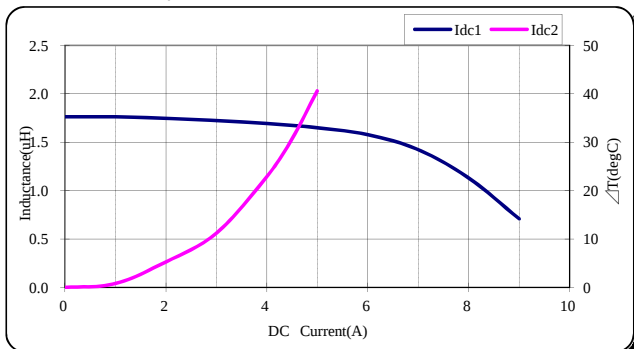
TDK' PartNo.;VLS5045EX-3R3N
