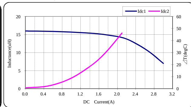
TDK' PartNo.;VLS5045EX-150M
