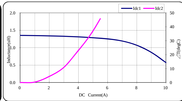
TDK' PartNo.;VLS5045EX-2R2N
