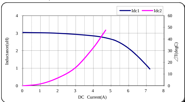
TDK' PartNo.;VLS5045EX-6R8M
