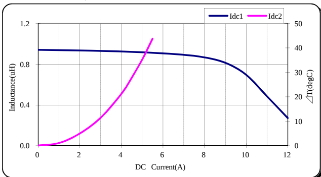
TDK' PartNo.;VLS5045EX-1R8N
