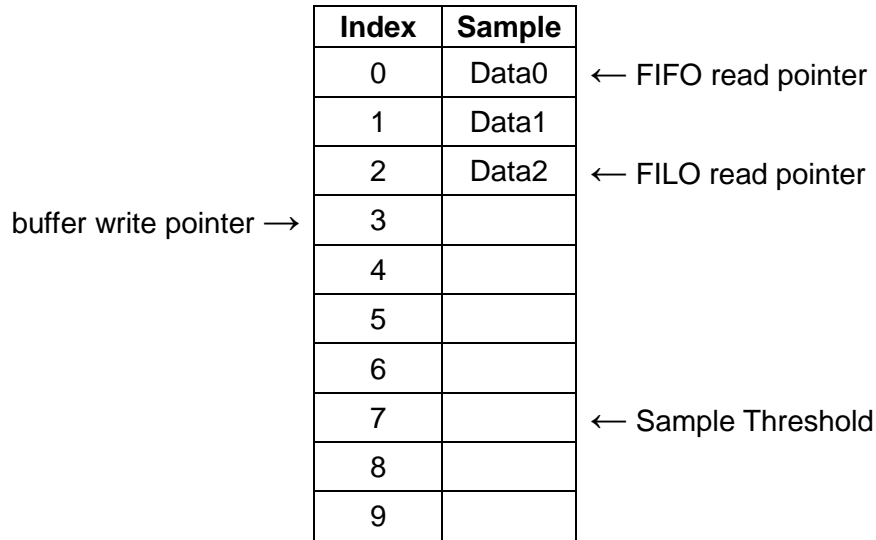
Figure 21: Buffer Filling
