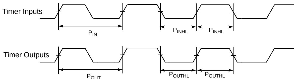
Figure 10-14 Timer Timing
