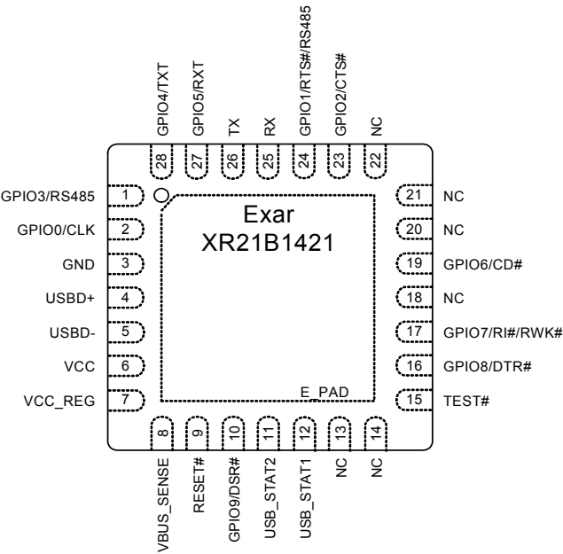
28-Pin Top View
