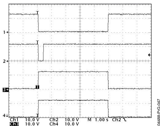
Figure 47. Timing Waveforms Associated with a RESTART Event (Ch1 = GATE; Ch2 = \overline{\text{RESTART}} ; Ch3 = PWRGD; Ch4 = SPLYGD)
