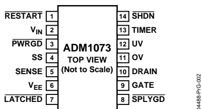
Figure 2. Pin Configuration
