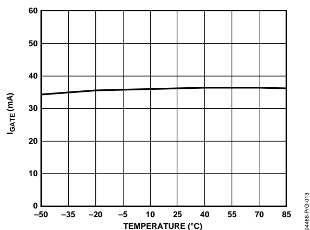
Figure 13. I_{GATE} (FCL, Sink) vs. Temperature ( V_{GATE} = 2 V)
