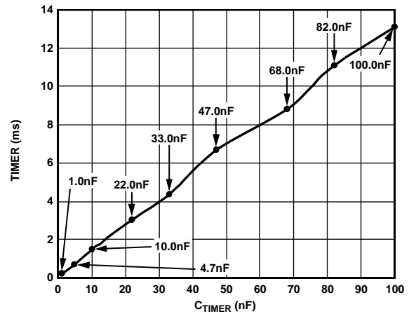
Figure 24. Current Limit On-Time vs. C_{TIMER} (1 nF – 100 nF)
