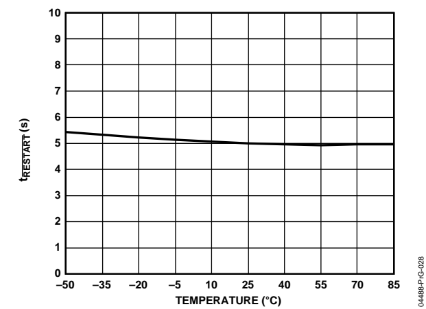
Figure 28. RESTART Time vs. Temperature
