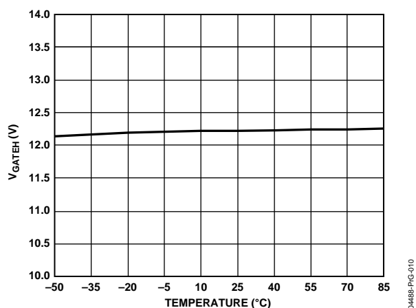
Figure 10. V_{GATEH} vs. Temperature
