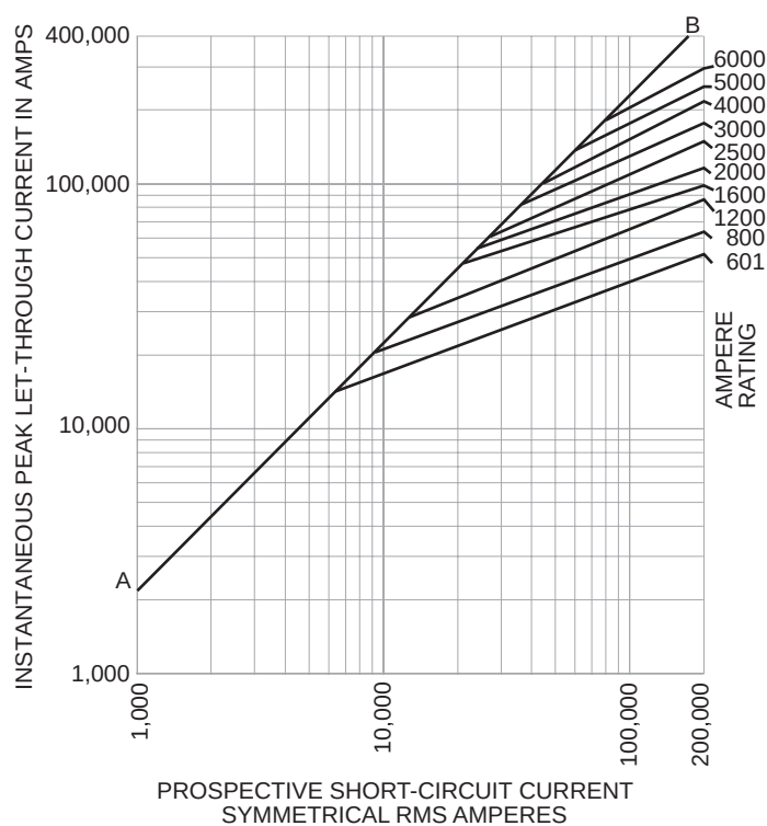
Current-Limitation Curves
