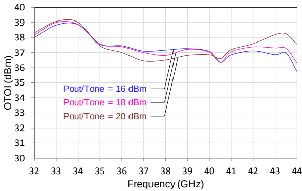
TOI vs. Pout/Tone vs. Frequency
