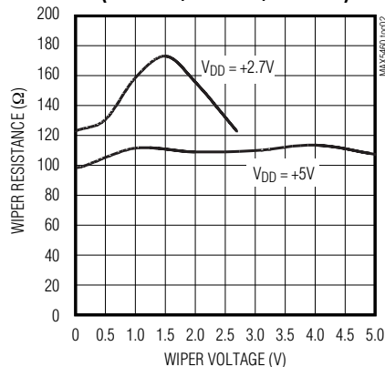
WIPER RESISTANCE vs. WIPER VOLTAGE (MAX5466/MAX5467/MAX5468)
