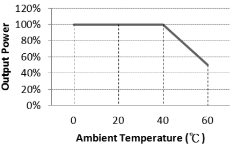
OUTPUT POWER DERATING CURVE
