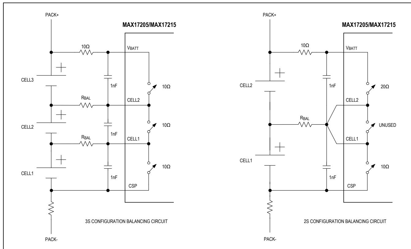
Figure 50. 2S and 3S Balancing Circuits
