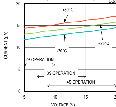
HIBERNATE CURRENT vs. SUPPLY VOLTAGE (MAX17205/MAX17215) toc04
