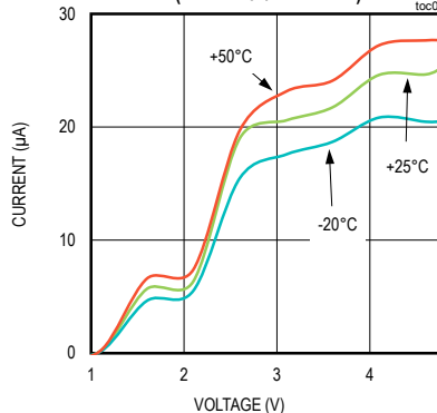
ACTIVE CURRENT vs. SUPPLY VOLTAGE (MAX17201/MAX17211) toc05
