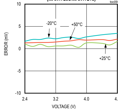
CELL2 VOLTAGE ADC ERROR (MAX17205/MAX17215) toc09
