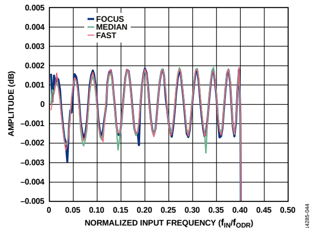
Figure 34. Wideband Filter Ripple
