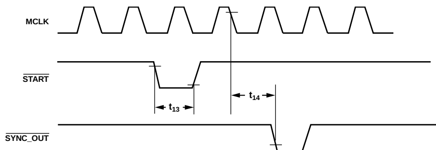
Figure 5. Asynchronous \overline{\text{START}} and \overline{\text{SYNC\_OUT}} Timing Diagram
