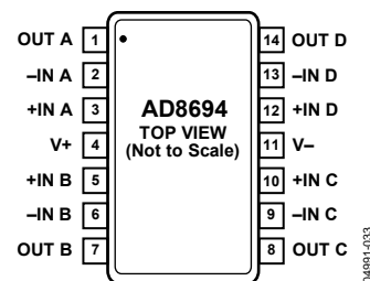
Figure 6. 14-Lead TSSOP
