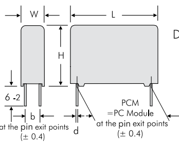
4-pin version
