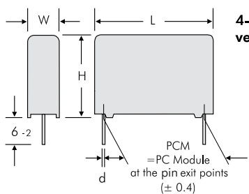
2-pin version
