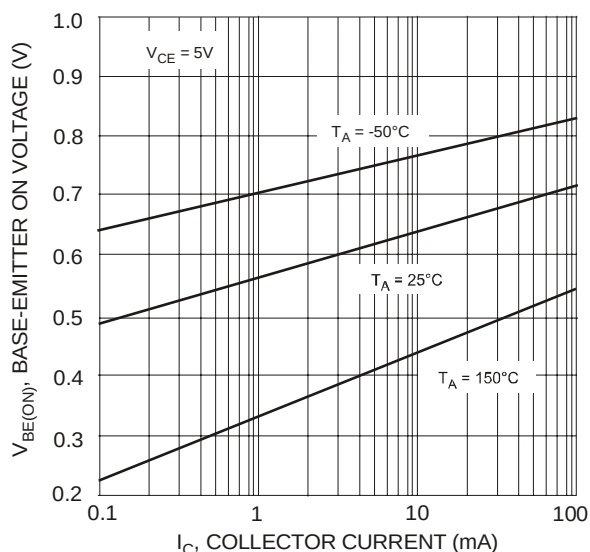
Fig. 14, Typical Base-Emitter On Voltage vs. Collector Current (DRDP006W)
