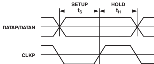
Figure 1. Setup and Hold Time
