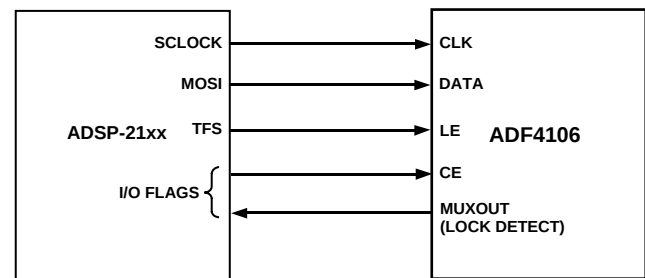
Figure 24. ADSP-21xx-to-ADF4106 Interface
