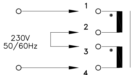
PRIMARY INPUT CONNECTIONS
