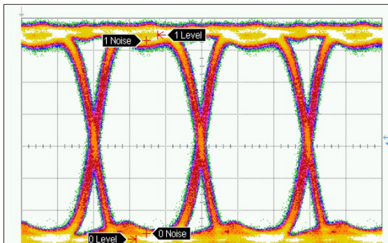
11.25 Gbps NRZ Output Eye Diagram
