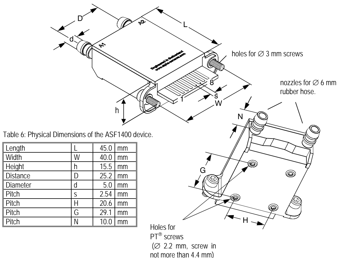
Figure 11: Physical dimensions and mounting information of the ASF1400.
