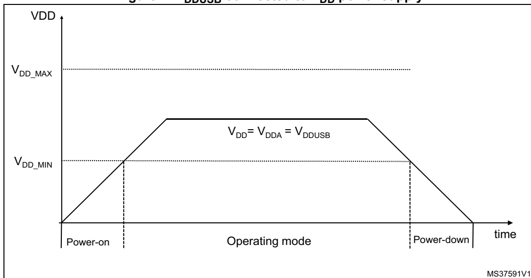
Figure 4. V DDUSB connected to V DD power supply
