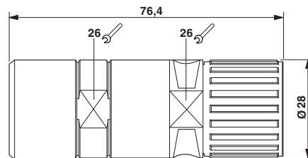
Dimensioned drawing
