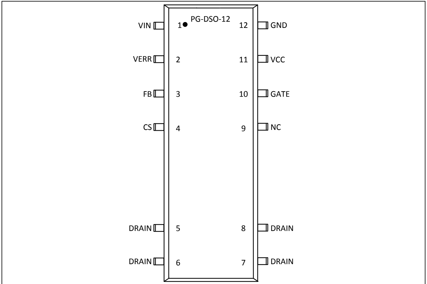
Figure 3 Pin configuration
