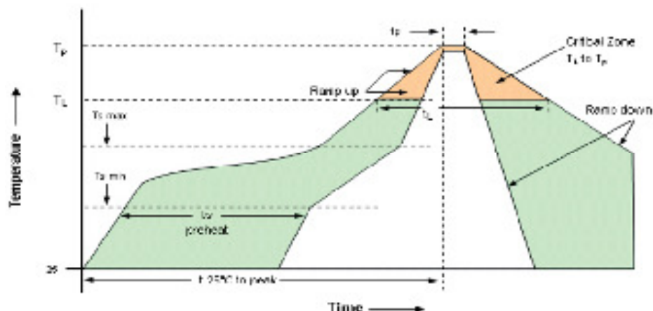
Figure 4. Recommended Reflow Profile
