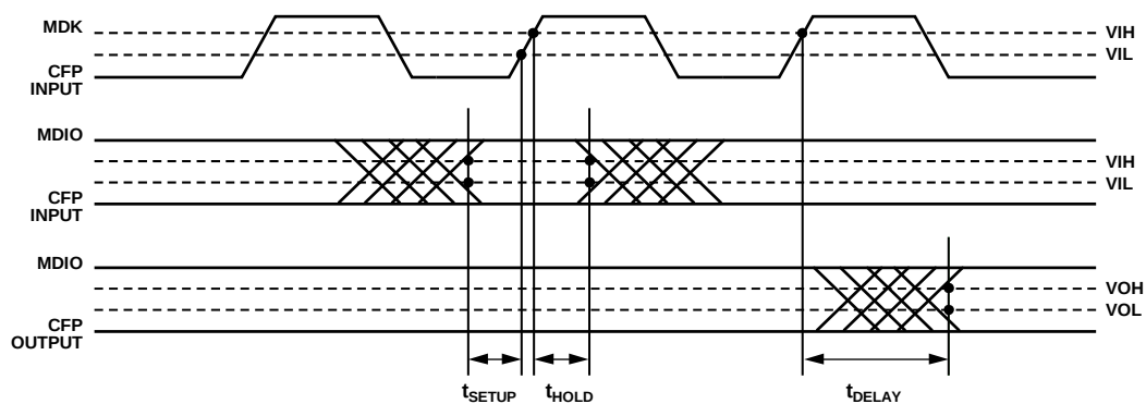
Figure 7. MDIO Timing
