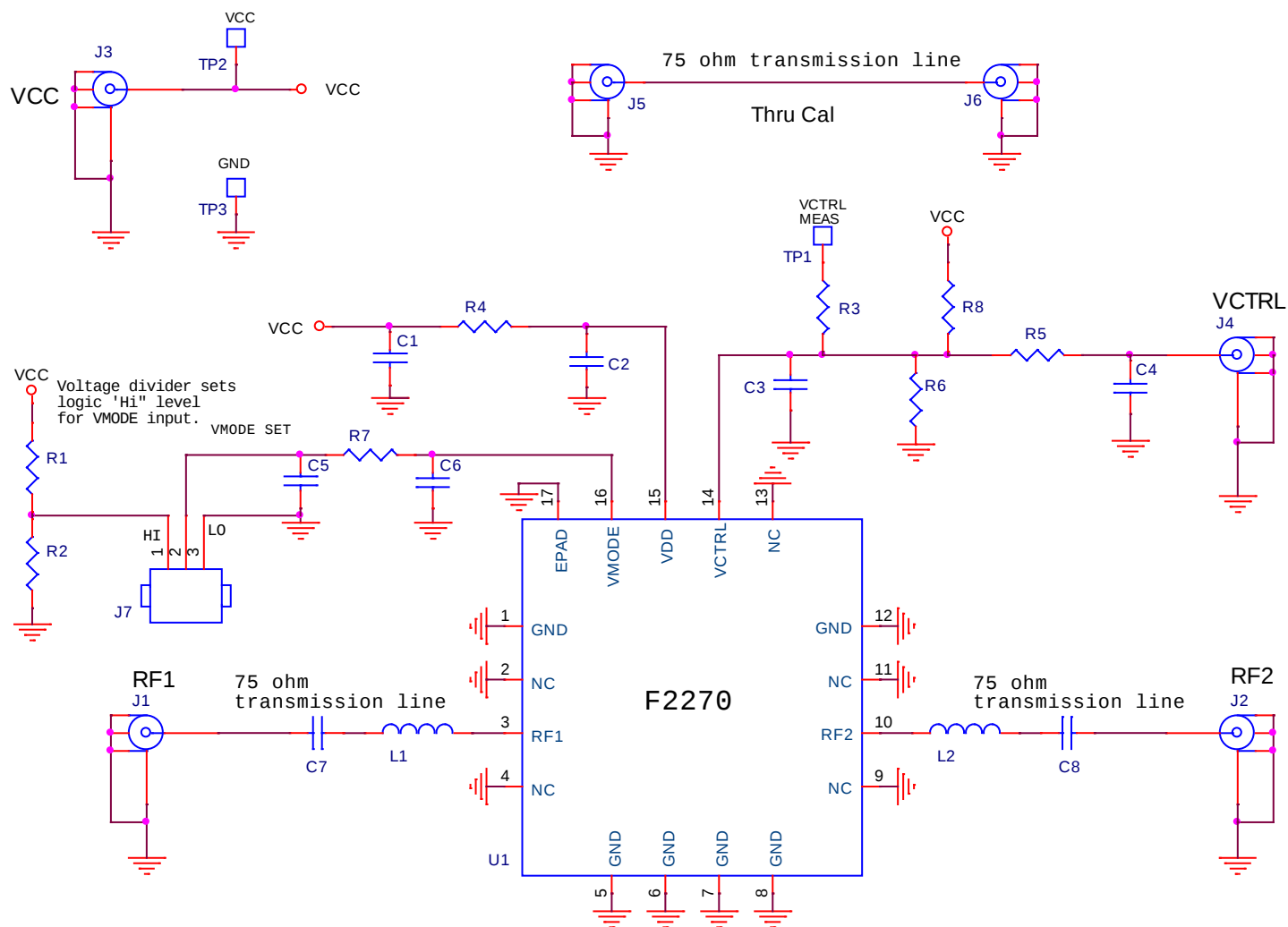
Figure 60. Electrical Schematic
