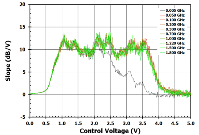
Figure 44. Attenuation Slope vs. V_{\text{CTRL}} [ V_{\text{MODE}} = \text{LOW} ]
