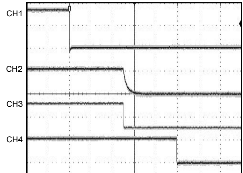
Shutdown of PWRHOLD and OUT3/5/6
