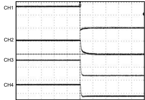
Shutdown of PWRHOLD and OUT11/10/8
