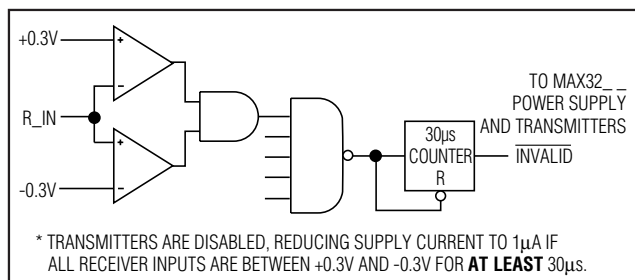
Figure 3a. MAX32_ _ Entering 1 \mu\text{A} Supply Mode via AutoShutdown
