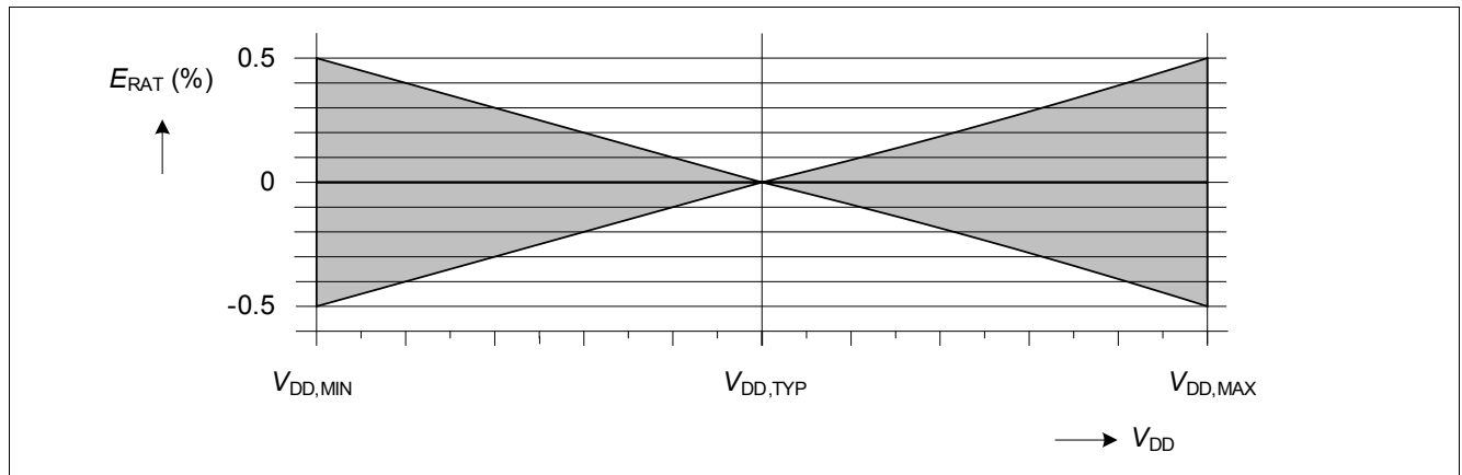
Figure 4 Ratiometric error
