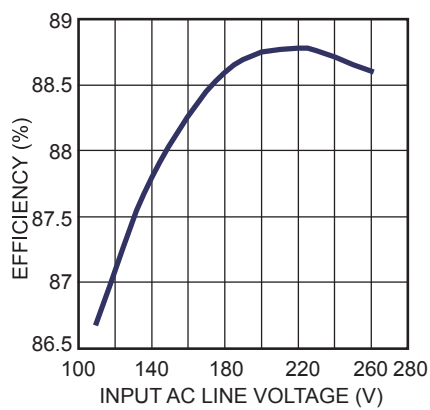
System Efficiency
