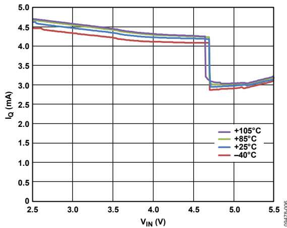
Figure 6. Typical Operating Current, G = 2x
