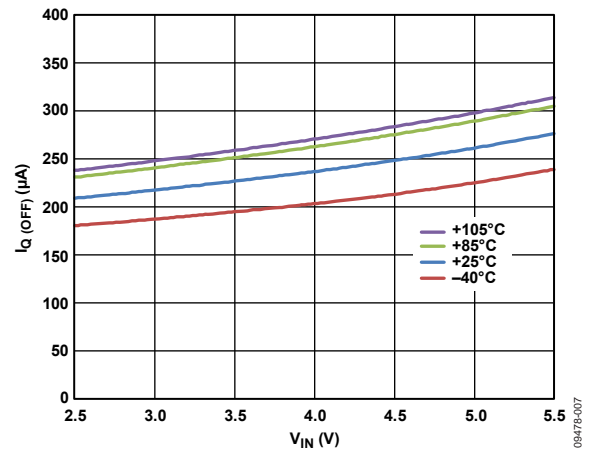
Figure 7. Typical Off Time Current ( I_{Q(\text{OFF})} )
