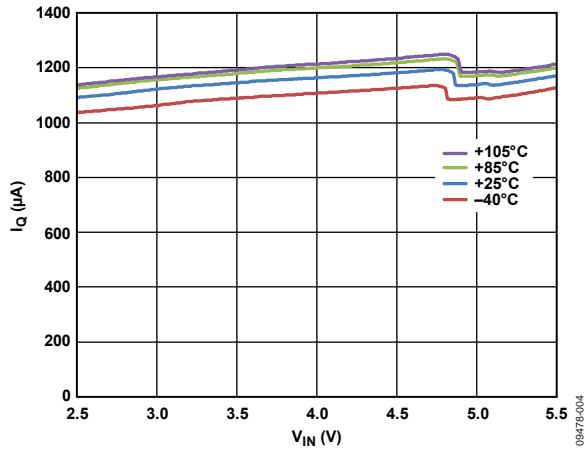
Figure 4. Typical Operating Current, G = 1x
