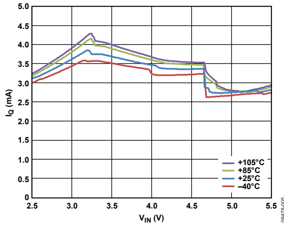
Figure 5. Typical Operating Current, G = 1.5x
