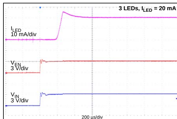
FIGURE 2-11: Start-Up When V_{IN} = V_{ENABLE} .
