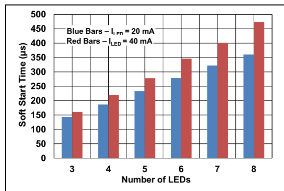
FIGURE 2-10: Soft Start Time vs. LED Number.
