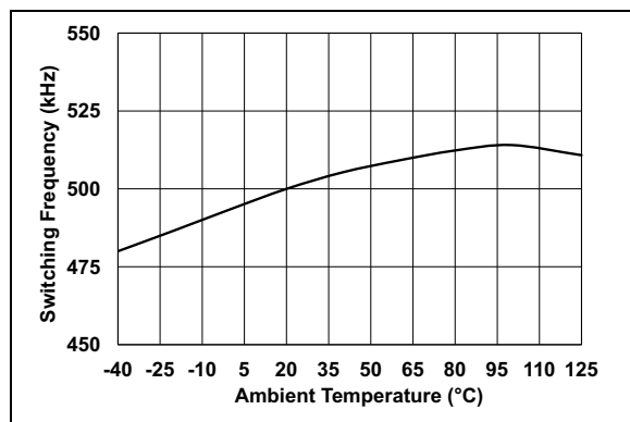
FIGURE 2-9: Switching Frequency, f_{SW} , vs. Ambient Temperature.
