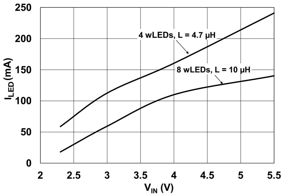
Maximum LED Current in Regulation vs. Input Voltage, T_A = 25^\circ C
