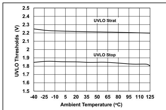
FIGURE 2-7: Undervoltage Lockout (UVLO) vs. Ambient Temperature.
