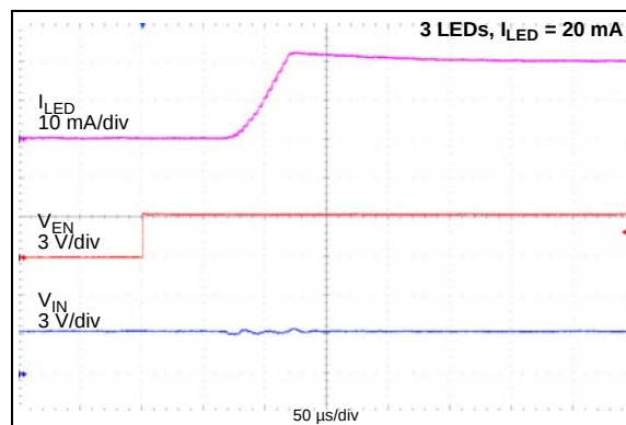
FIGURE 2-12: Start-Up After Enable.
