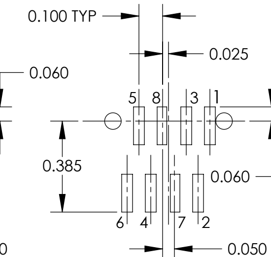
(8 PIN) SURFACE MOUNT TRASM8M1X TRASM8MX
