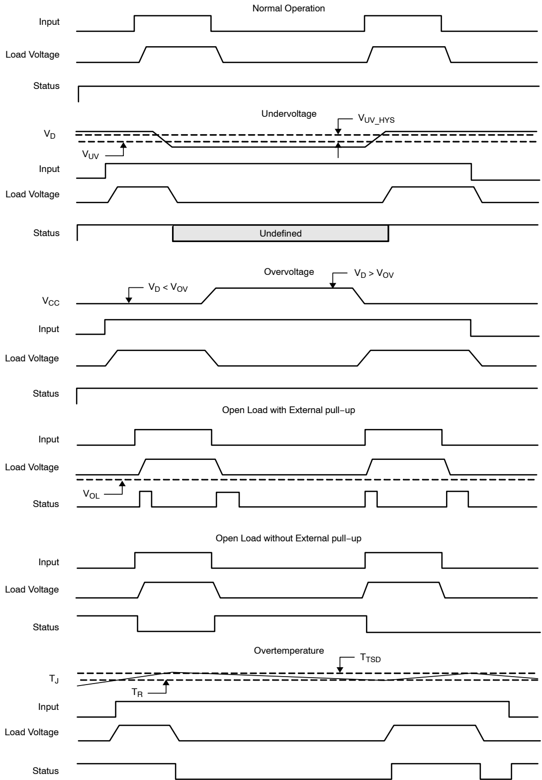
Figure 30. Waveforms
