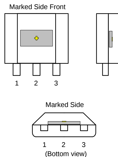
Figure 19. SIP (LPG) Package
