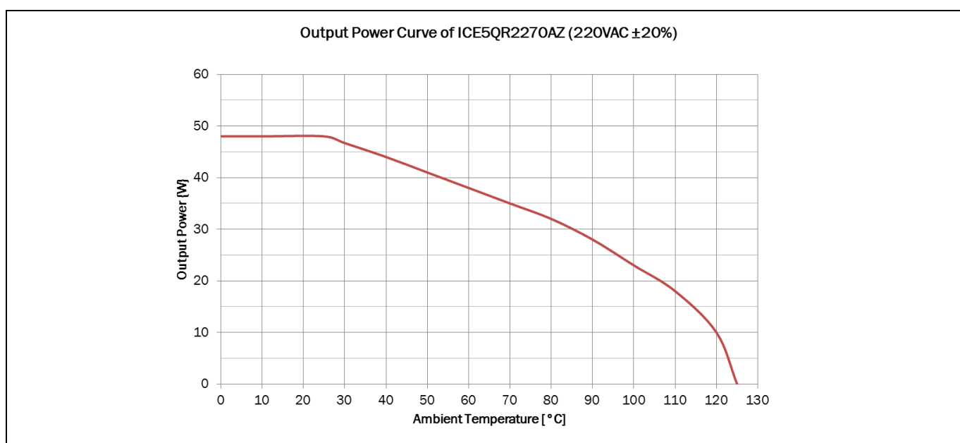
Figure 46 Output power curve of ICE5QR2270AZ, V_{IN}=220\text{ V}_{AC} ; P_{Out}=f(T_a)
