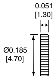
COVER
