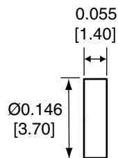
INSULATOR
