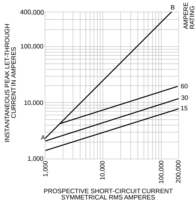
Current-Limitation Curves
