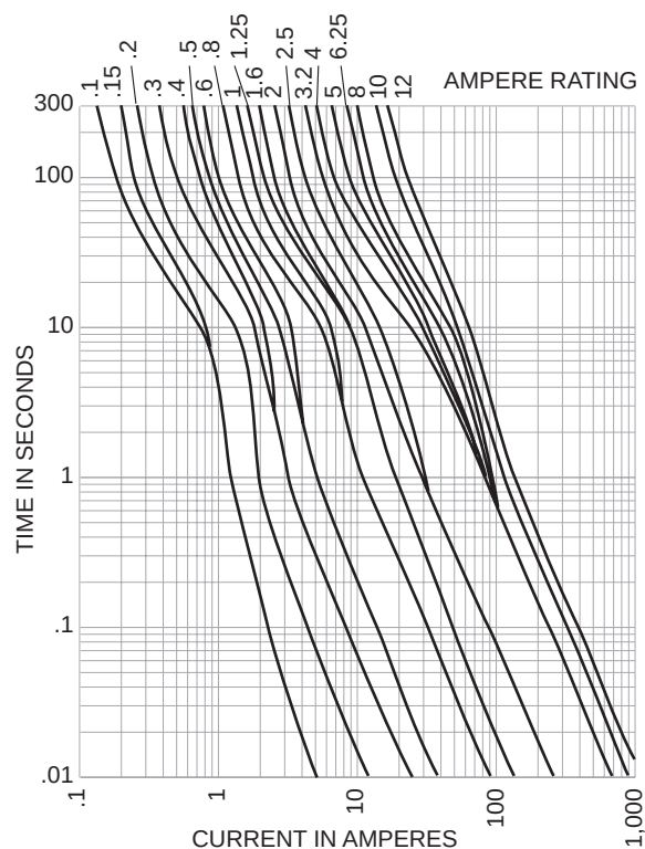
Current-Limitation Curves
